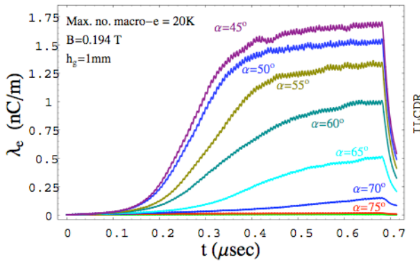
Figure 2: E-cloud accumulation during passage of a 0.68 \mu\text{sec} bunch train for various steepness angles of triangular (sharp edge) grooves.
