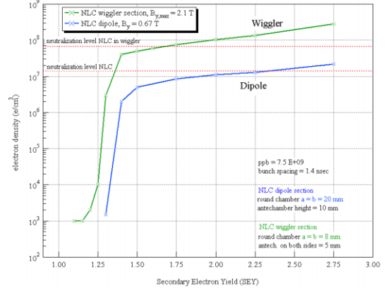
Figure 5: Saturation density as a function of \delta_{\max} in a NLC wiggler (above) and a dipole section. Thresholds for the development of the electron cloud are respectively \delta_{\max} \sim 1.3 and 1.4. Note that the neutralization level in a wiggler is higher due to a smaller beam pipe cross section.
