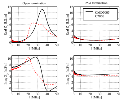
Figure 4: Comparison of bench-measured coupling impedance for open and 25 \Omega PFN termination, and high (1600) and medium (100) permeability ferrite.
