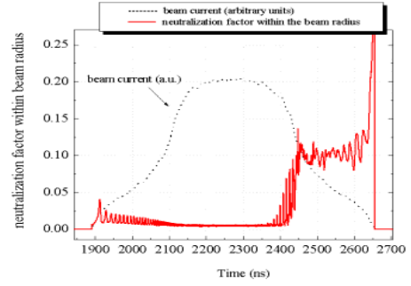
Figure 3: Simulation of single-bunch electron multipacting with a peak secondary-emission yield of 2.
