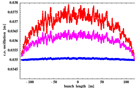
Figure 2: Orbit deviation for 3 turns due to beam-centroid offset from the mechanical center of the extraction kickers.
