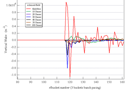
Figure 4: Long-range wake function due to electron cloud for bunch spacing S_b = 3S_{RF} .
