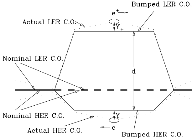
Figure 1: Elevation sketch of the vertical closed orbit bump near the IP (LER=low-energy ring, HER=high-energy ring).
