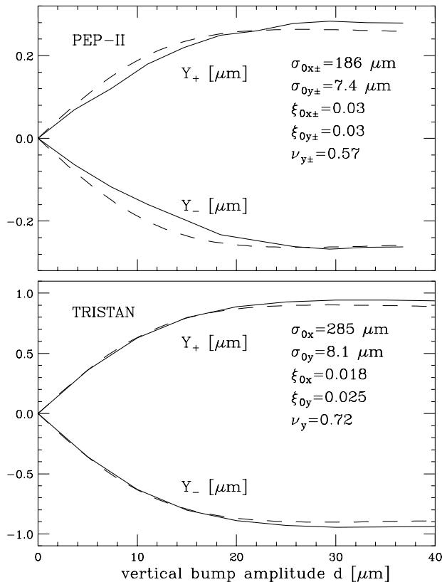
Figure 2: Beam-beam induced orbit offset at the IP for PEP-II and TRISTAN. Solid: multiparticle simulations; dashed: result from solving Eqs. (1–2) for nominal parameters.
